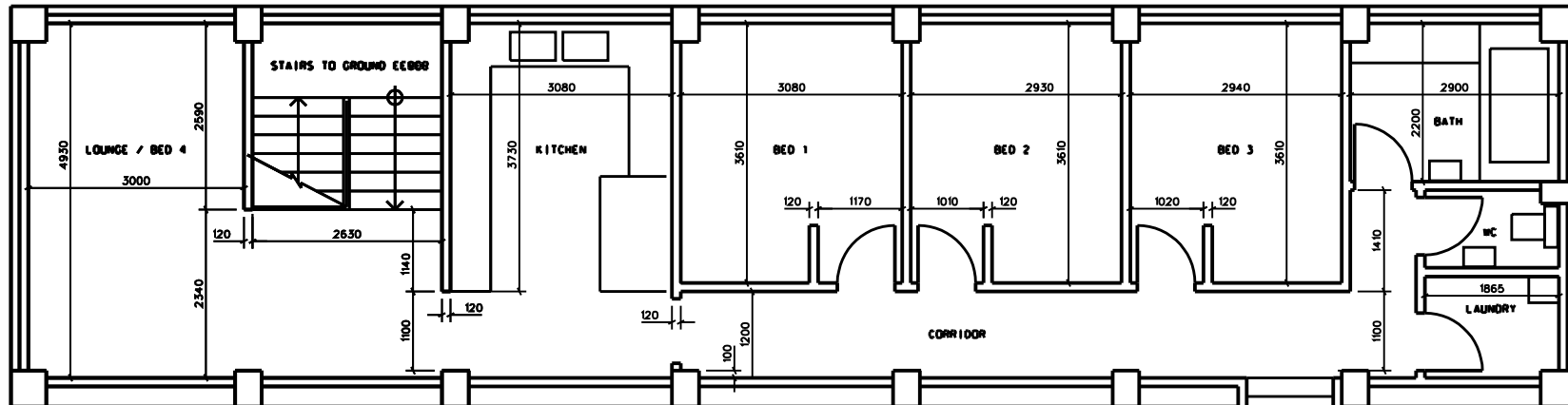
FIRST FLOOR
